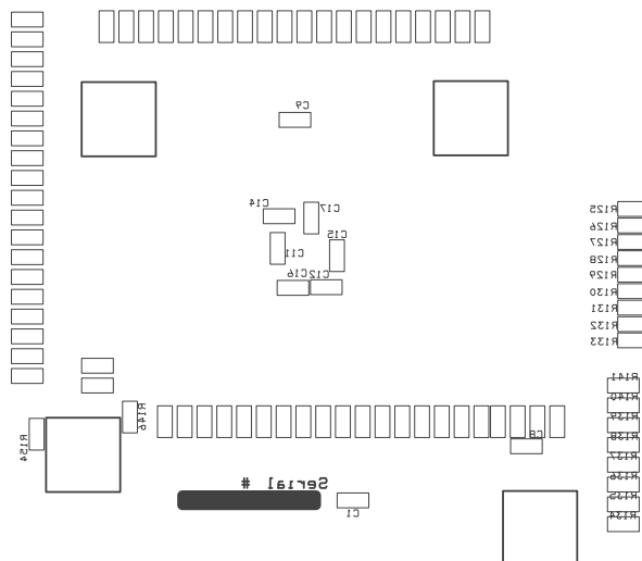
Figure 4. Bottom Silkscreen
