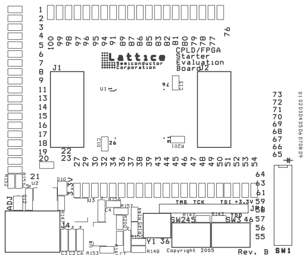
Figure 1. Top Silkscreen
