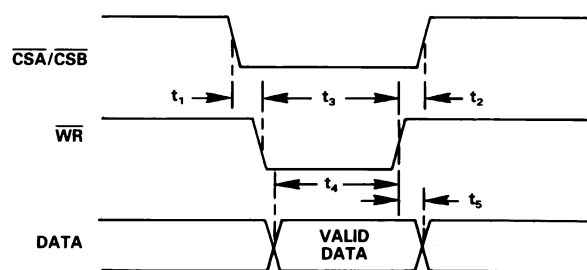
Figure 5. AD7247A Write Cycle Timing Diagram
