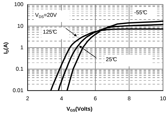
Figure 3: Transfer Characteristics
