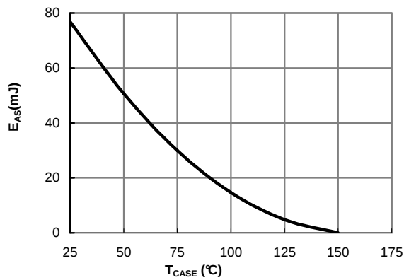
Figure 14: Avalanche energy
