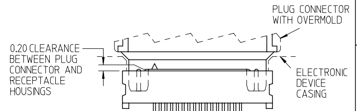
RECOMMENDATIONS FOR CONFIGURATION OF MATED CONNECTORS
