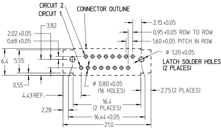
PCB HOLE LAYOUT (CONNECTOR MOUNTING SIDE)
