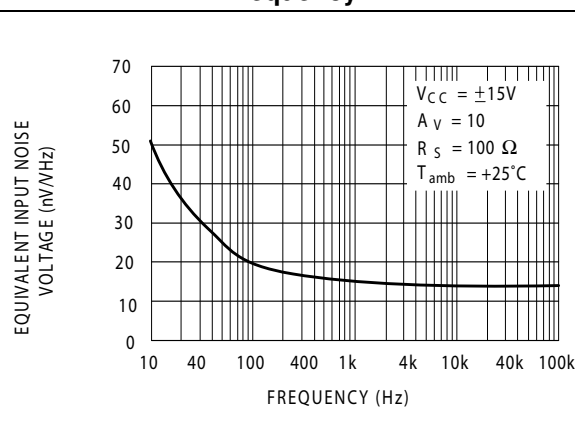
Figure 17. Equivalent input noise voltage vs. frequency
