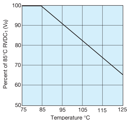
Category Voltage vs. Temperature
