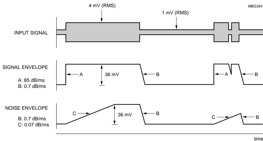
Fig.10 Signal and noise envelope waveforms.
