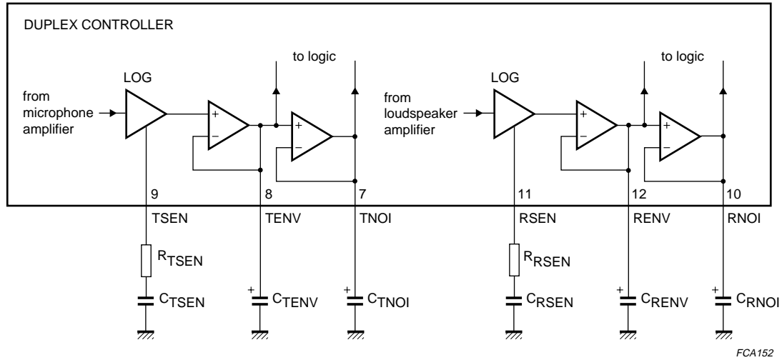
Fig.9 Signal and noise envelope detectors.
