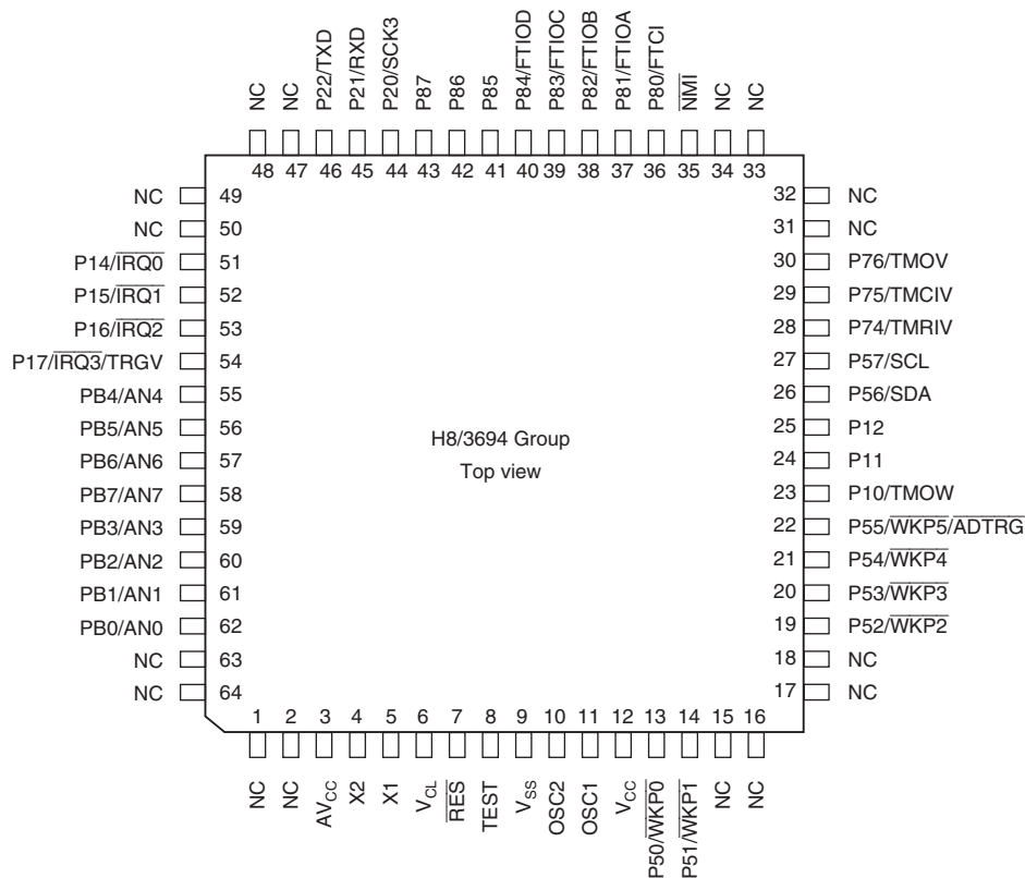
Figure 1.3 Pin Arrangement of H8/3694 Group of F-ZTAT TM and Mask-ROM Versions (FP-64E, FP-64A)
