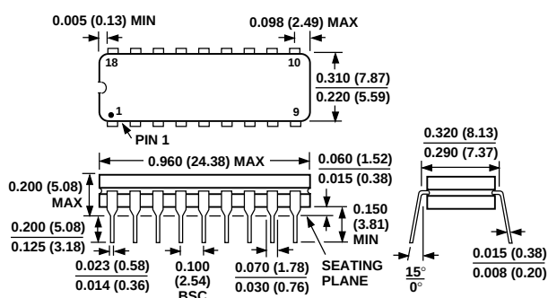
18-Lead Cerdip (Q-18)
