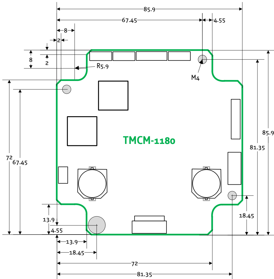
Figure 4.1: Dimensions of TCMC-1180 and mounting holes
