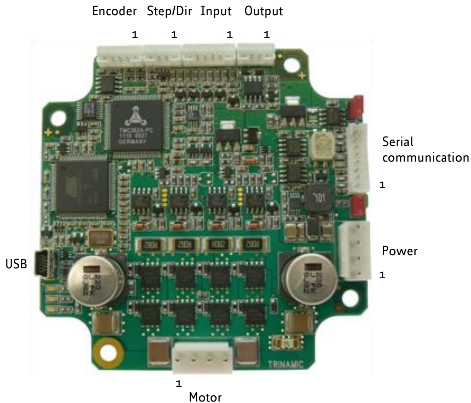
Figure 4.4: Overview connectors
