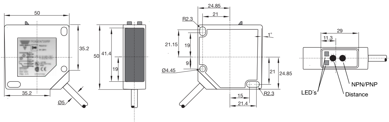
Cable version
