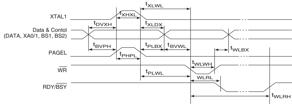
Figure 24-7. Parallel Programming Timing, Including some General Timing Requirements
