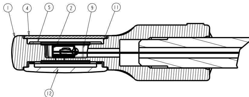
SECTION B-B SCALE 4:1
