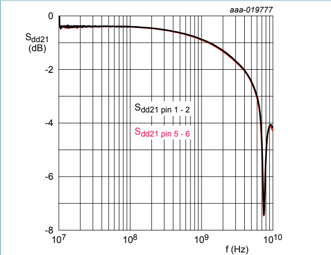
Fig. 1. Differential-mode insertion loss; typical values
