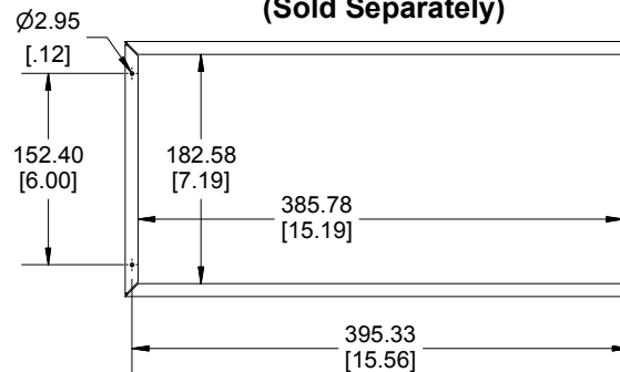
Bottom View of Chassis (Sold Separately)
