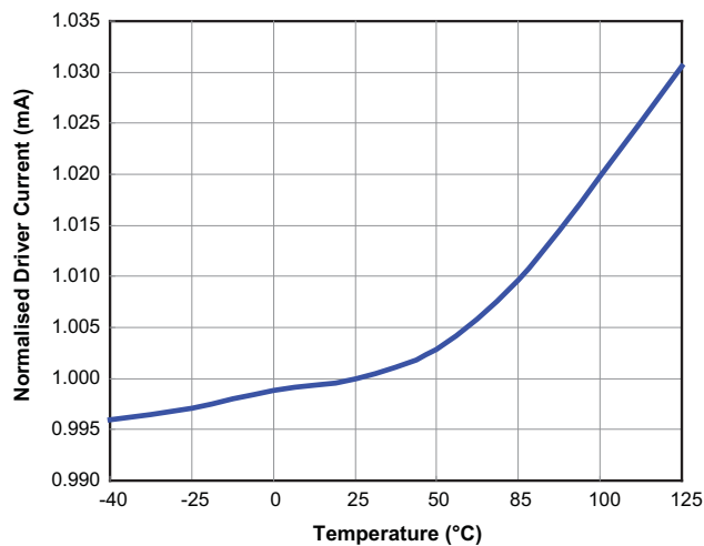
Fig 8. I_{DRV} + I_{VCIN} vs. Temperature
