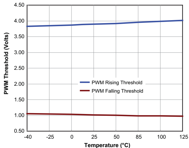
Fig 10. PWM Input Threshold vs. Temperature
