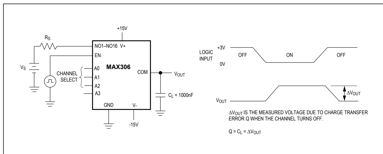
Figure 5. Charge Injection
