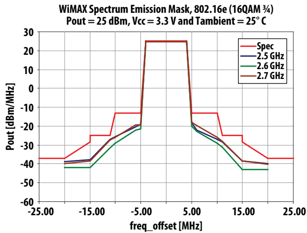
Figure 17. SEM Frequency Sweep at Vcc = 3.3 V and 25°C (2 dB Post-PA loss assumed)
