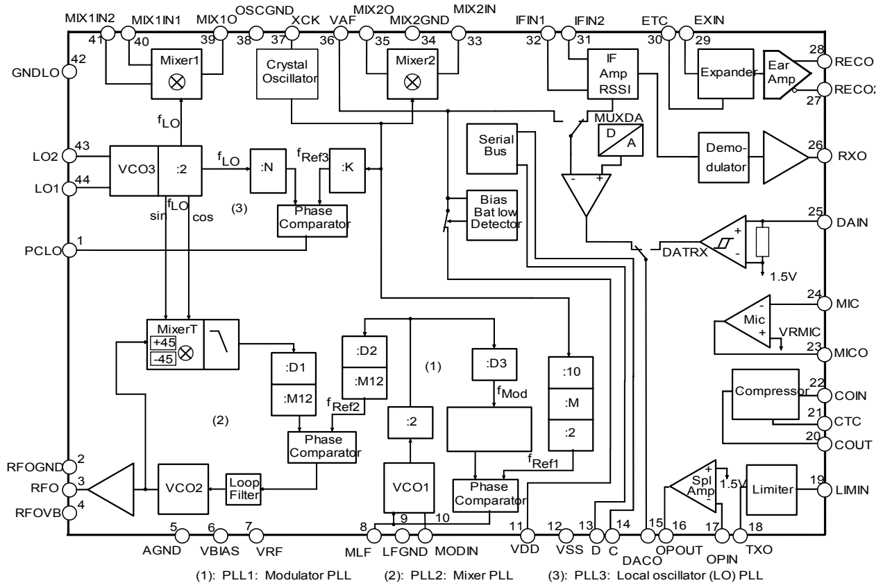
Figure 1-1. Block Diagram
