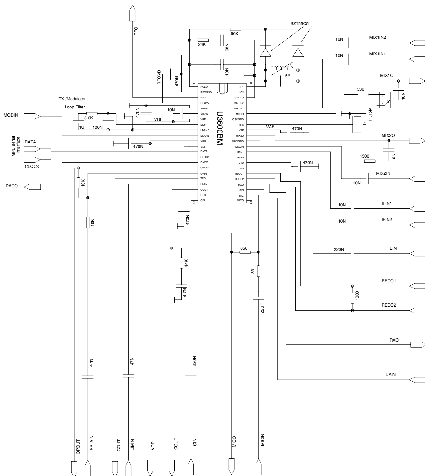
Figure 8-1. Test Circuit
