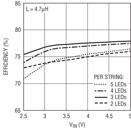
LED Efficiency vs V_{IN}
