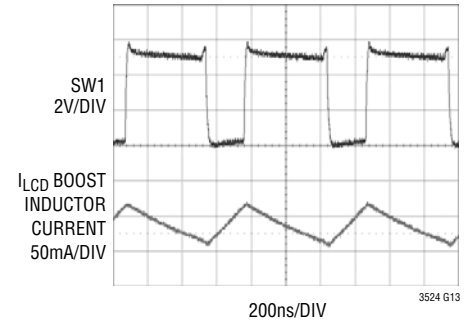
SW1 Voltage and 10 \mu H Inductor Current at 25mA Load
