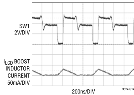
SW1 Voltage and 10 \mu H Inductor Current at 5mA Load
