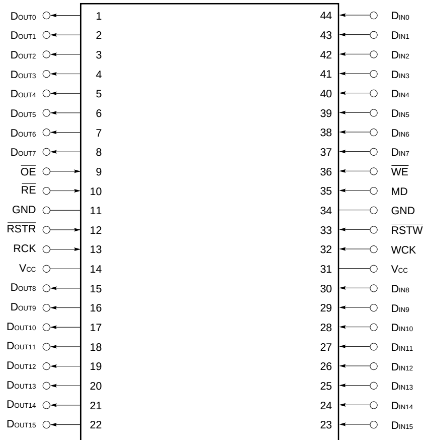
44-pin plastic TSOP (II) (10.16 mm (400)) [μPD485506G5-7JF]
