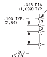
PC MOUNTING
