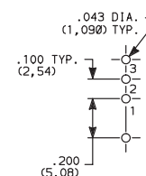
PC MOUNTING
