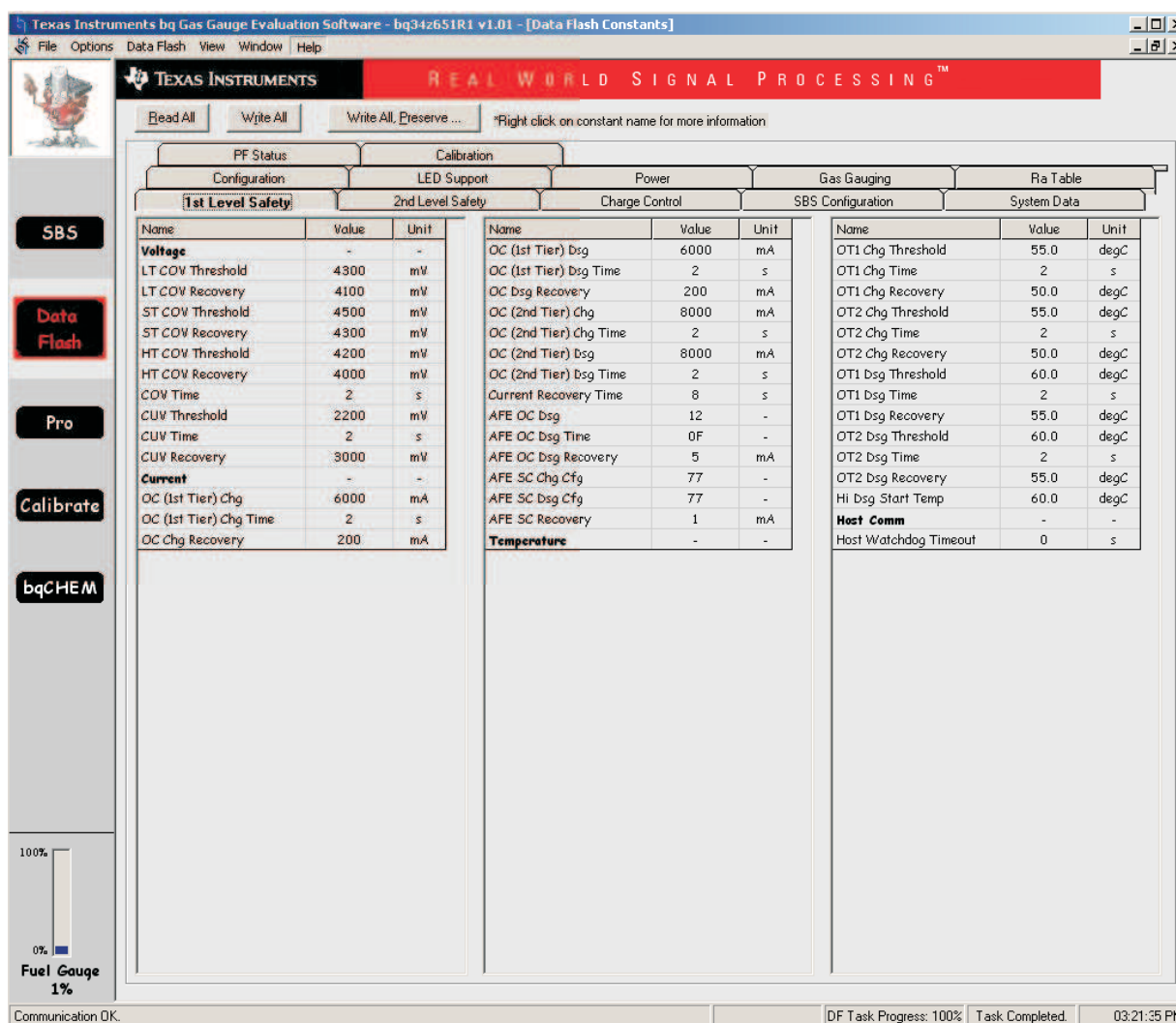
Figure 9. Data Flash Screen, 1st Level Safety Class
