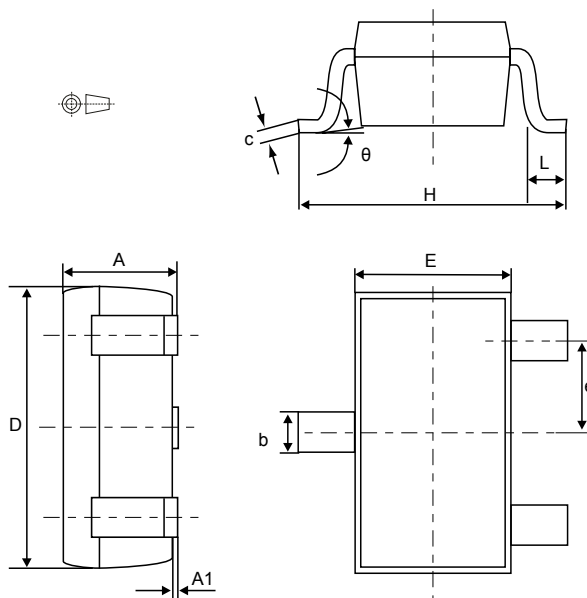
Figure 15. SOT323-3L package outline
