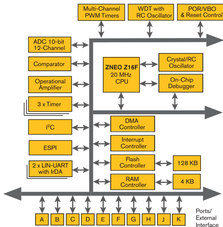
ZNEO Z16F Block Diagram & System Flow Chart
