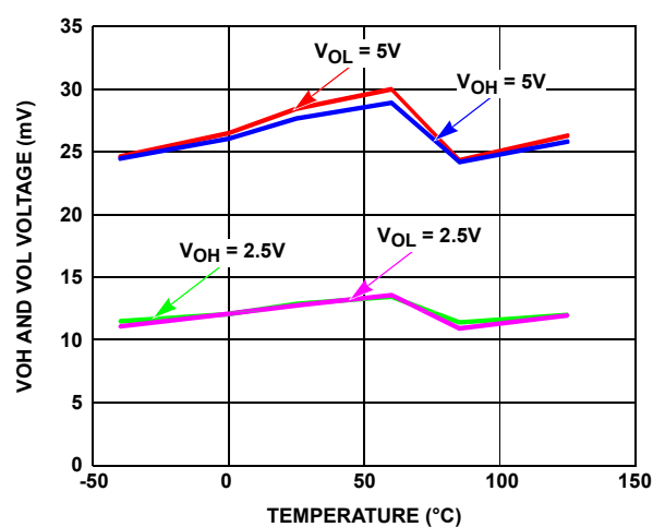
FIGURE 60. OP AMP V_{OH} AND V_{OL} vs TEMPERATURE
