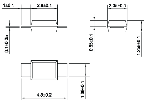
Lead design 1
