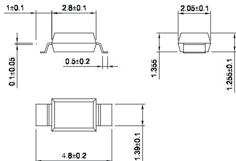
Lead design 2
