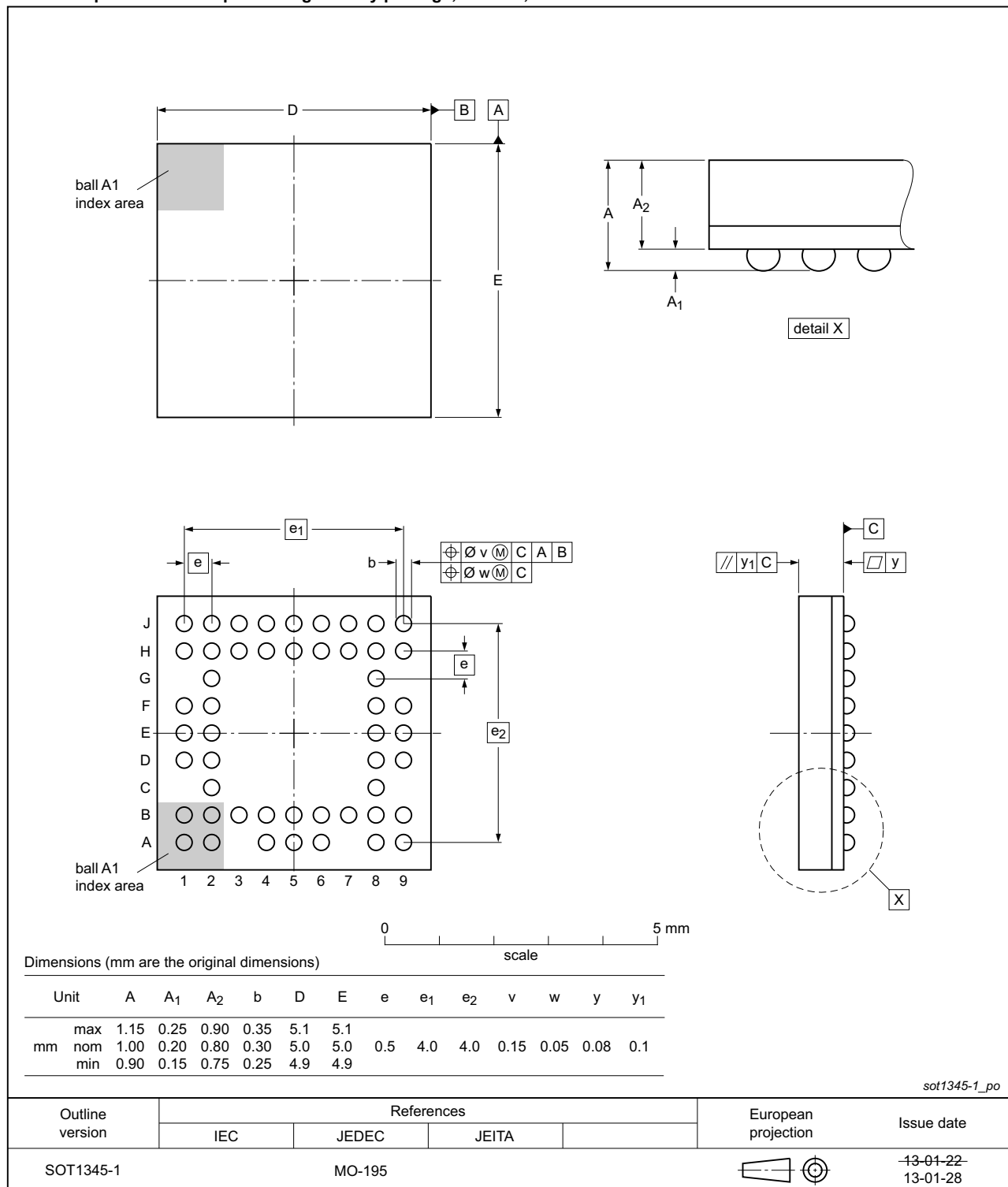
Fig 5. Package outline TFBGA50 (SOT1345-1)
