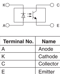
Internal Circuit
