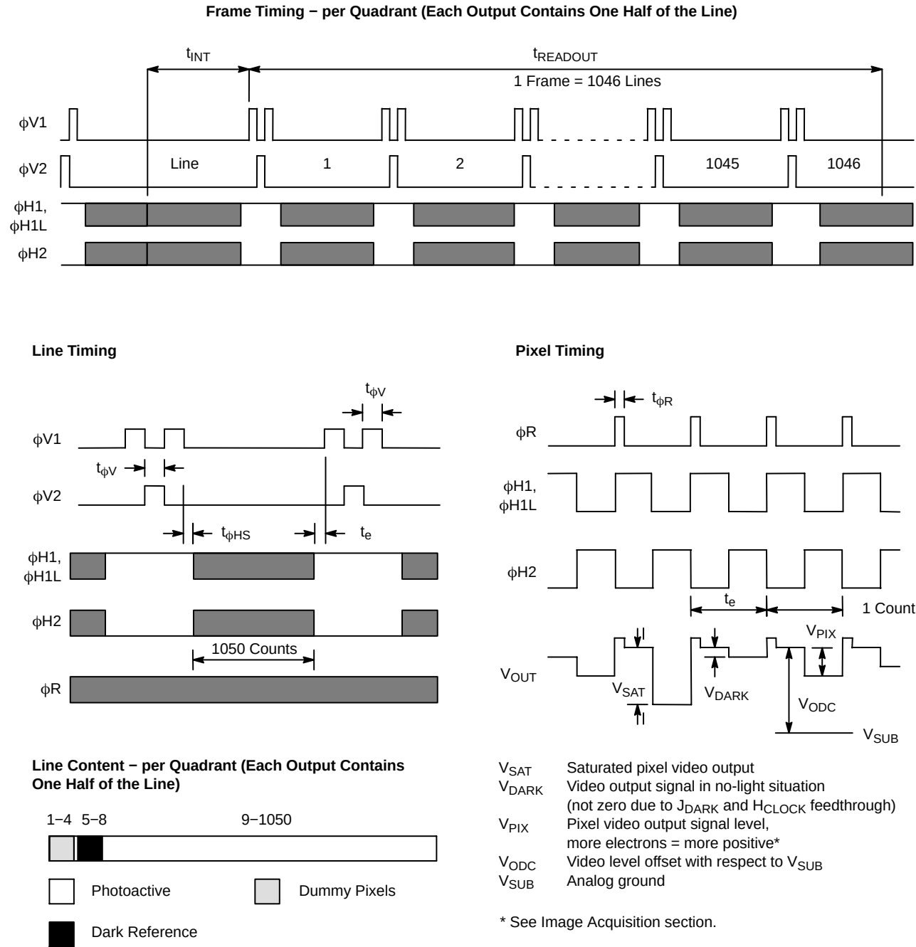
Figure 17. Timing Diagrams
