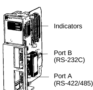
C200HW-COM06-E
