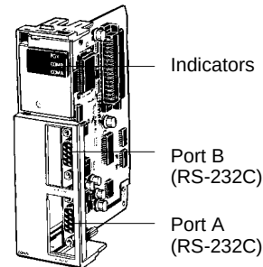
C200HW-COM05-E
