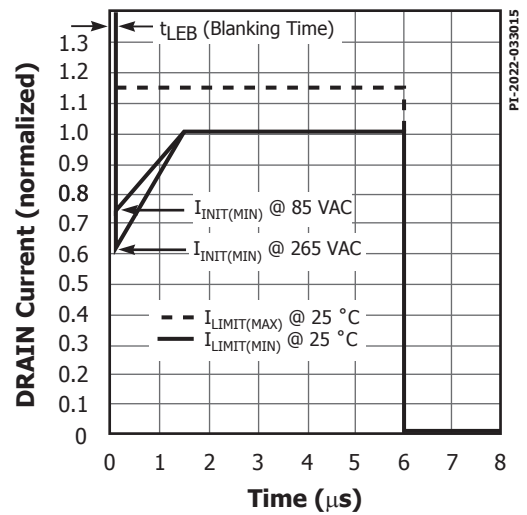
Figure 33. Drain Current Operating Envelope.
