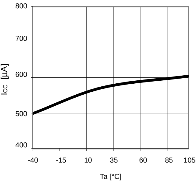
Figure 22. T_a - I_{\text{CC}}
