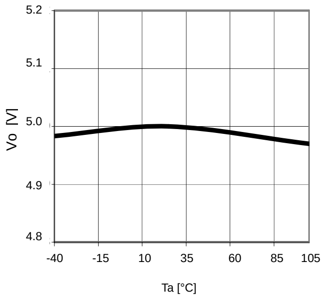
Figure 21. T_a - V_{\text{O}} ( I_{\text{O}}=0\text{mA} )
