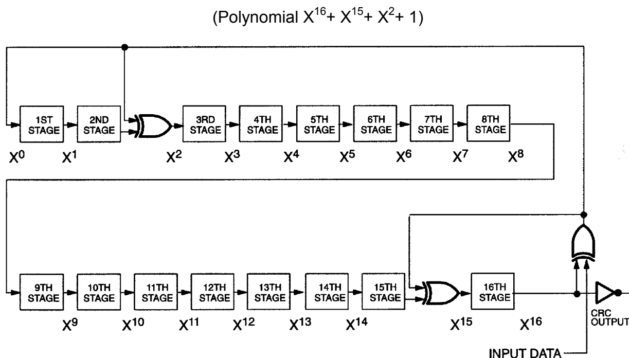
Figure 12. CRC-16 HARDWARE DESCRIPTION AND POLYNOMIAL
