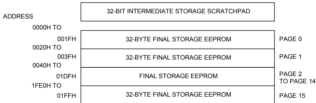
Figure 5. DS2433 MEMORY MAP
