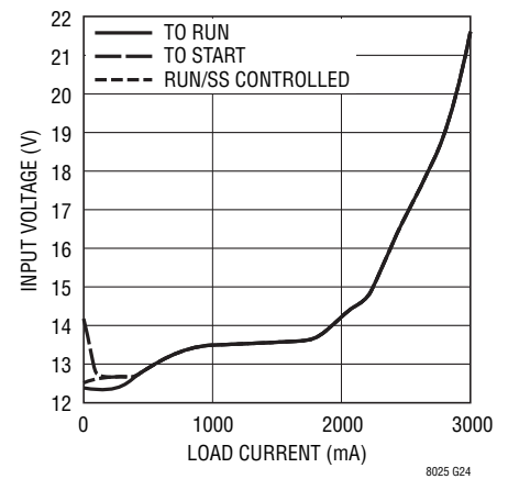
Minimum Input Voltage vs Load Current, 12V_{OUT}
