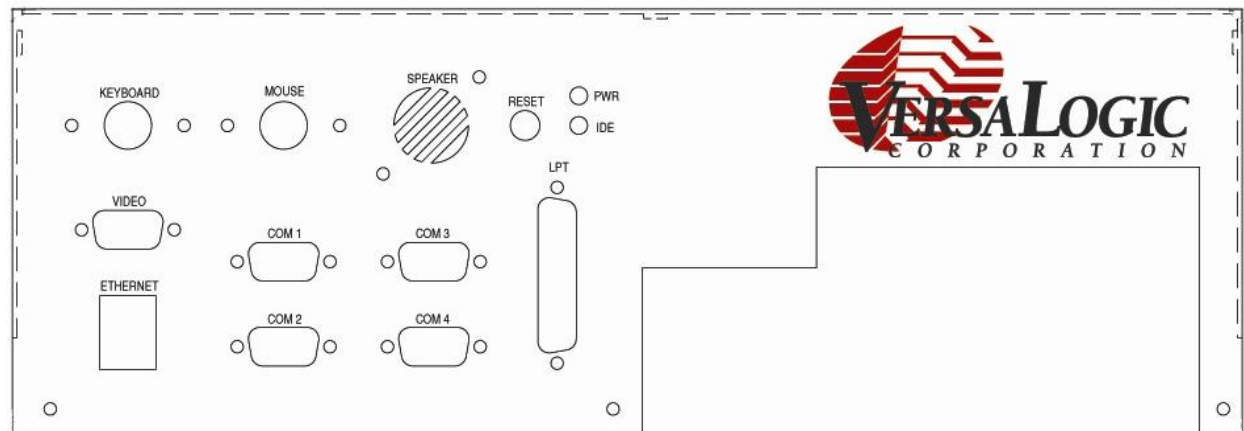
Figure 2. VL-ENCL-5B Front Panel
