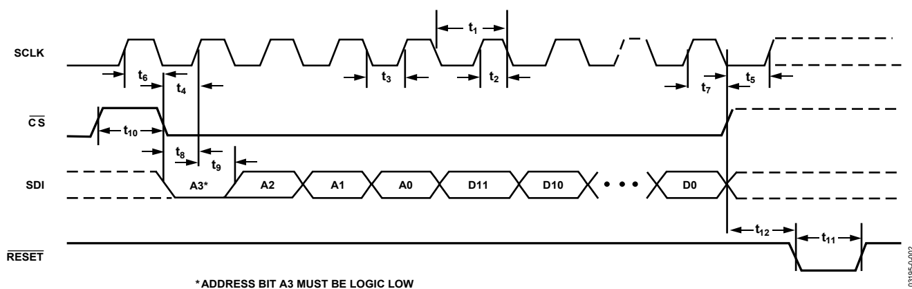
Figure 2. Timing Diagram
