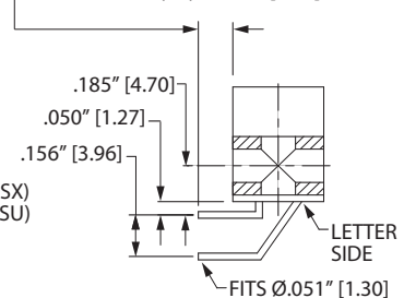
RIGHT ANGLE, DIP SOLDER (RA, SA)
