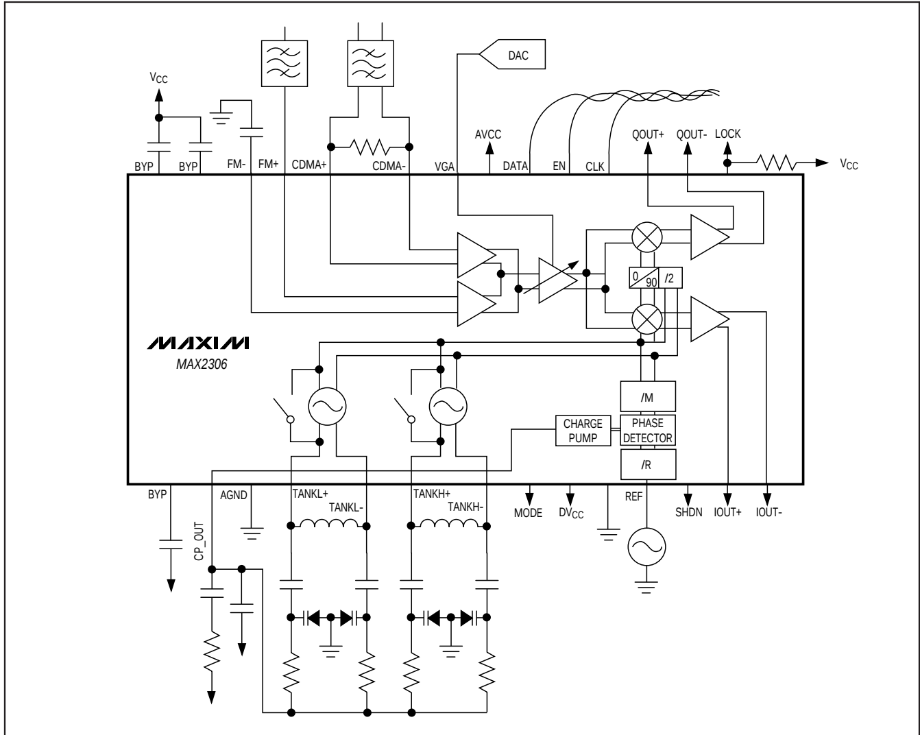
Block Diagram
