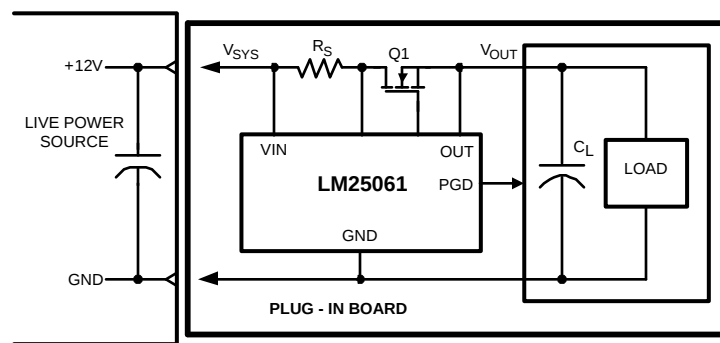
Figure 22. LM25061 Application
