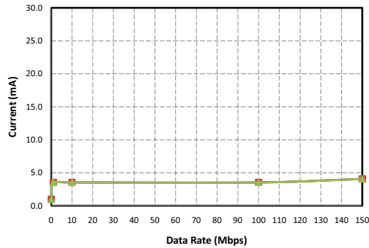
Figure 9. Si8640/45 Typical V_{DD1} Supply Current vs. Data Rate 5, 3.3, and 2.5 V Operation
