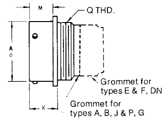
Crimp KPSE01/MS3121
