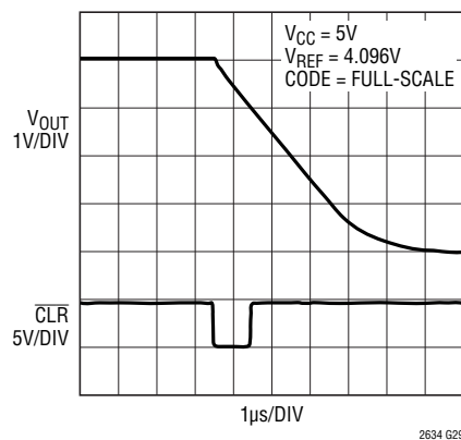
Hardware \overline{\text{CLR}}
