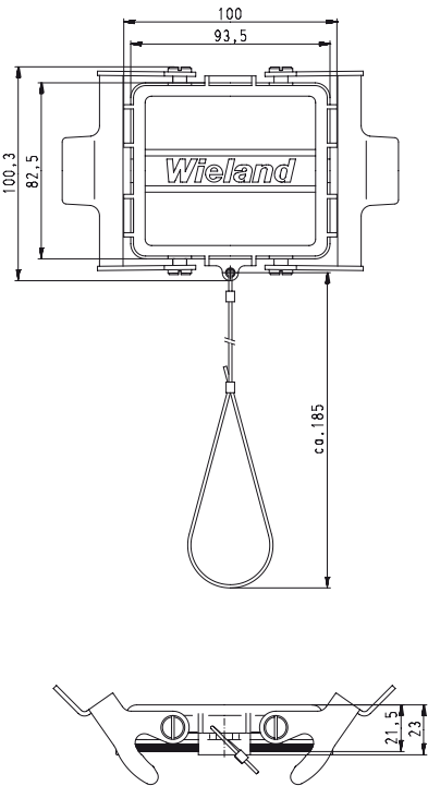
Protective cover with locking levers
