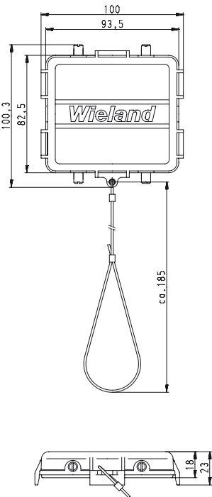
Protective covers without locking levers
