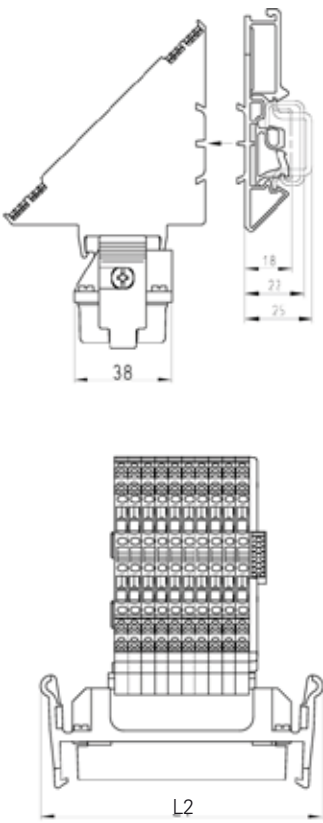
with locking levers
