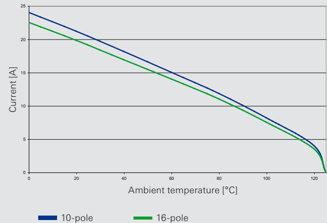
Derating curve according to IEC 60512 sec. 3 revos HD 10/16 250 V / 16 A / 1.5 mm 2
