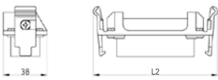
with locking levers without strain relief
