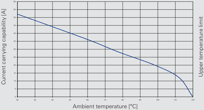
Derating curve according to IEC 60512 sec. 3 revos POWER 70.200/210.0653.0 revos POWER 6-pole 400 V / 35 A / 6.0 mm 2
