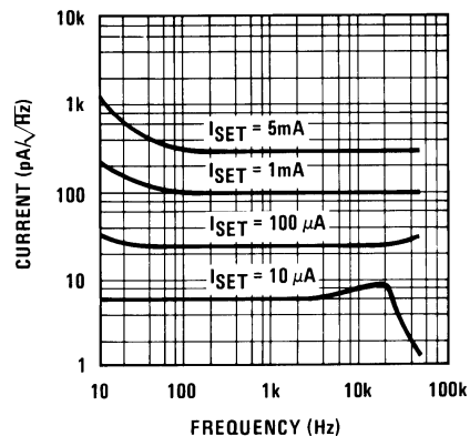
Current Noise
