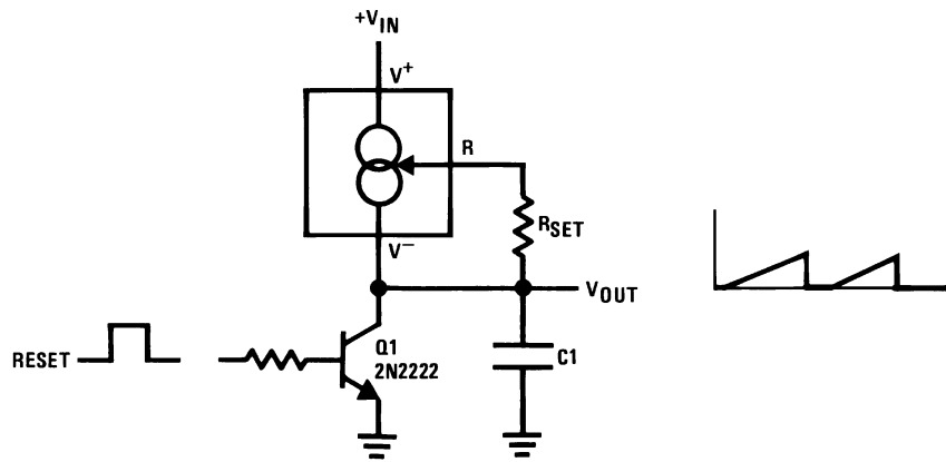
Ramp Generator
