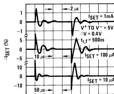
Transient Response
