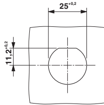
Dimensioned drawing
