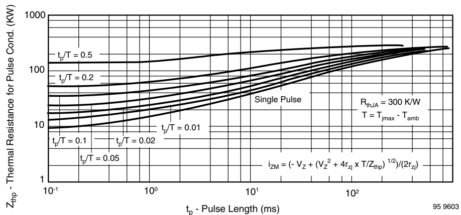
Fig. 13 - Thermal Response
