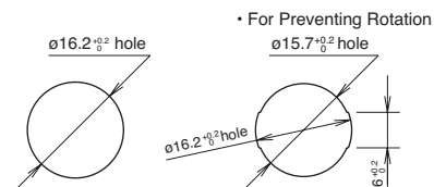
Mounting Hole
