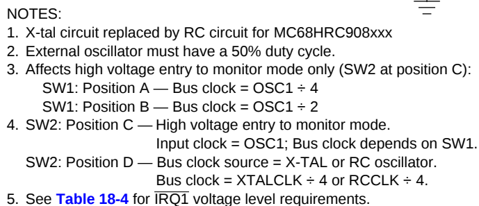
Figure 9-1. Monitor Mode Circuit
