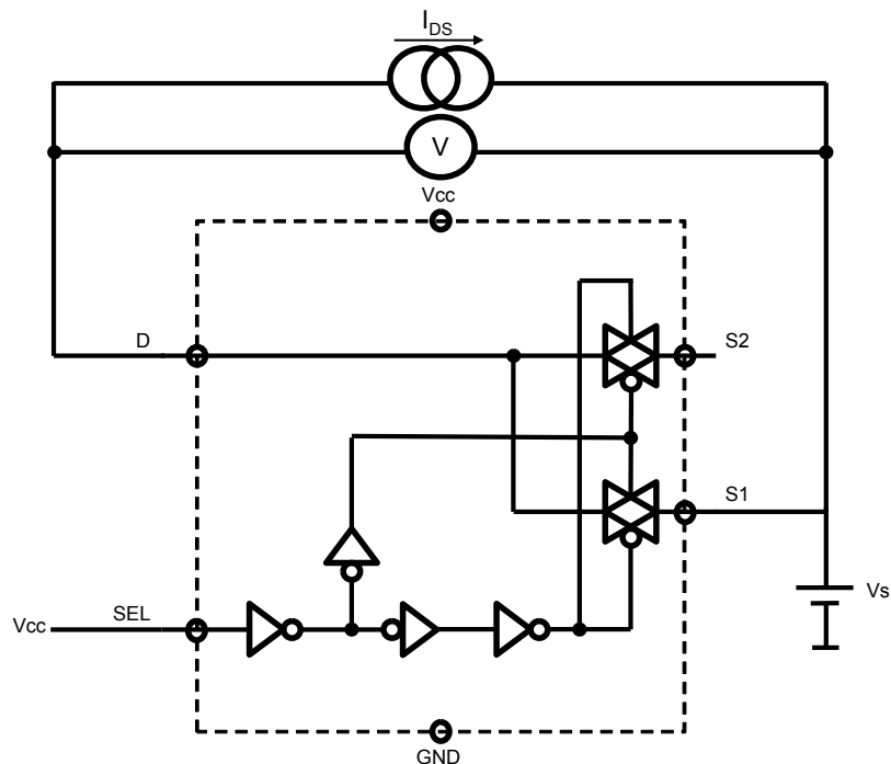
Figure 3. On-resistance
